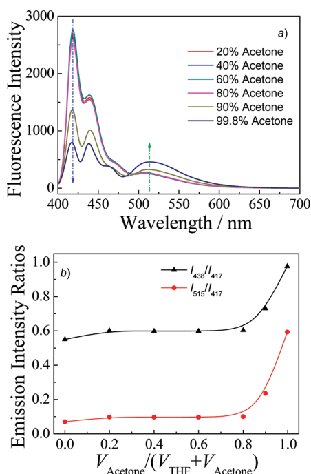
Figure 1. (a) Fluorescence emission spectra and (b) fluorescence intensity ratio changes (Ex. 5 nm; Em. 5 nm, \lambda_{\text{ex}} = 390 nm) recorded for P(MMA- co -NBDAE) 56 - b -PF 9 - b -P(MMA- co -NBDAE) 56 triblock copolymer in THF/acetone mixture (0.1 g/L; [PF] = 6.58 \mu\text{M} , [NBDAE] = 3.68 \mu\text{M} ) with increasing volume fractions of acetone.
