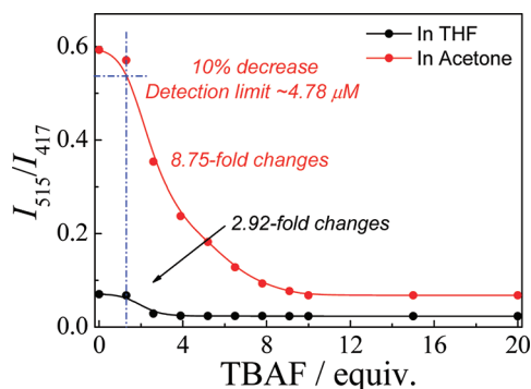
Figure 3. Fluorescence emission intensity ratio changes recorded for P(MMA-co-NBDAE) 56 -b-PF 9 -b-P(MMA-co-NBDAE) 56 micelles in acetone and unimers in THF (0.1 g/L, [PF] = 6.58 μM, [NBDAE] = 3.68 μM), respectively, upon addition of 0–20 equiv of TBAF (Ex. 5 nm; Em. 5 nm, λ ex = 390 nm).
