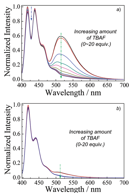
Figure 2. Fluorescence spectra recorded for P(MMA- co -NBDAE) 56 - b -PF 9 - b -P(MMA- co -NBDAE) 56 triblock copolymer (a) micelles in acetone and (b) unimers in THF (0.1 g/L, [PF] = 6.58 \mu\text{M} , [NBDAE] = 3.68 \mu\text{M} ), respectively, upon addition of 0–20 equiv of TBAF (Ex. 5 nm, Em; 5 nm, \lambda_{\text{ex}} = 390 nm).
