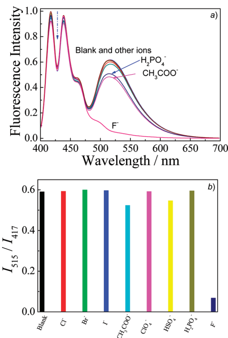
Figure 4. (a) Fluorescence spectra and (b) fluorescence intensity ratio changes of micellar solution of P(MMA-co-NBDAE) 56 -b-PF 9 -b-P(MMA-co-NBDAE) 56 triblock copolymer in acetone (0.1 g/L, [PF] = 6.58 μM, [NBDAE] = 3.68 μM) in the presence of 10 equiv (20 μL acetone solution) of tetra- n -butylammonium (TBA) salts of Cl − , Br − , I − , CH 3 COO − , ClO 4 − , HSO 4 − , H 2 PO 4 − , and F − (Ex. 5 nm; Em. 5 nm, λ ex = 390 nm).
